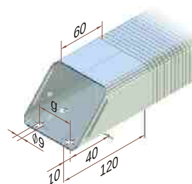
scoop bracket
